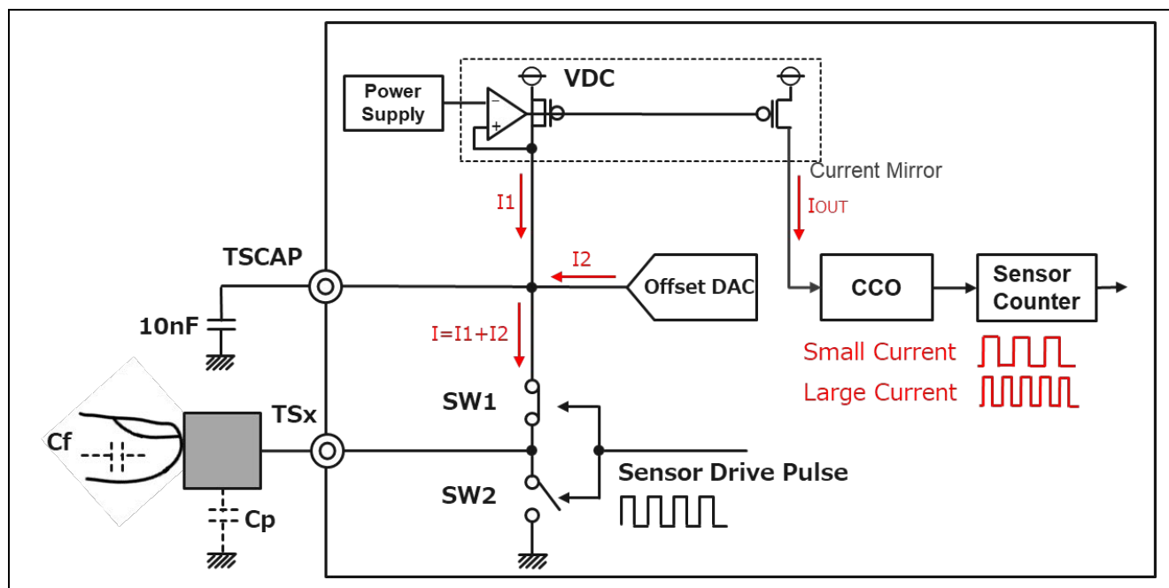
Figure 2.3 Measurement circuit of CTSUS
