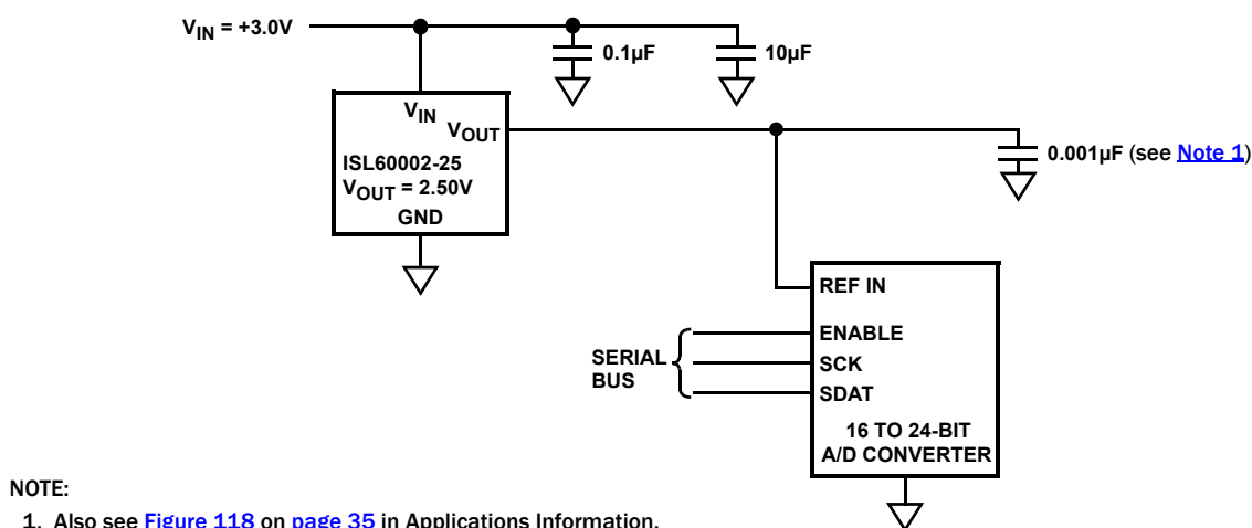
FIGURE 1. TYPICAL APPLICATION
