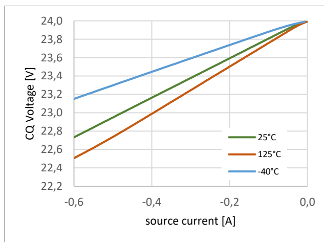
Figure 10. C/Q Driver High Voltage vs. Source Current
