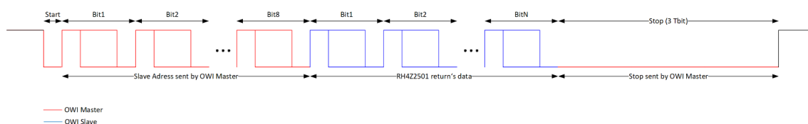
Figure 25: OWI Read Command Chronogram
