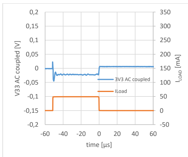
Figure 12. V33 LDO Transient Load Response
